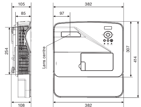
Unit: mm
